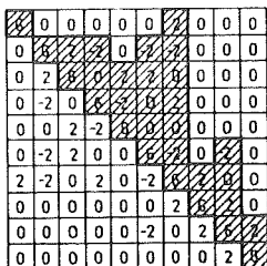
Fig.2 Profile of matrix Q (hatched)
