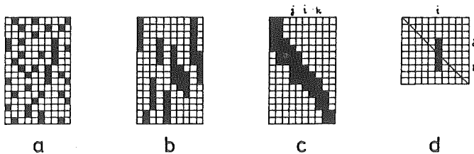
Fig.3 a. the original matrix A b. A after completion of the first step (row interchanges) c. A after second step (column interchanges) d. i -th column of the matrix Q formed from rearranged A (c.) (Blackened areas contain nonzero elements)
